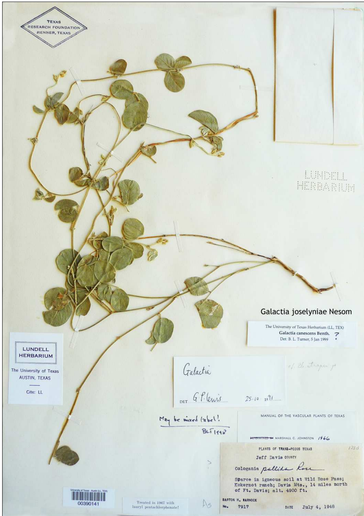
Figure 12. Galactia joselyniae . Warnock 7917 (LL), from Wild Rose Pass in Jeff Davis Co., Texas.
