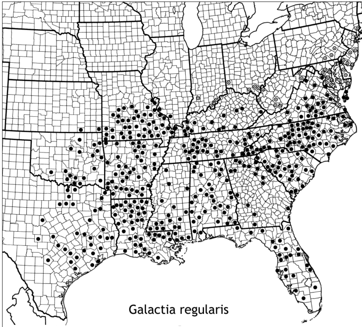
Map 11. Northern records without specimens examined in the present study added from various sources — because there is no other species of Galactia in this area, the identifications seem secure.
